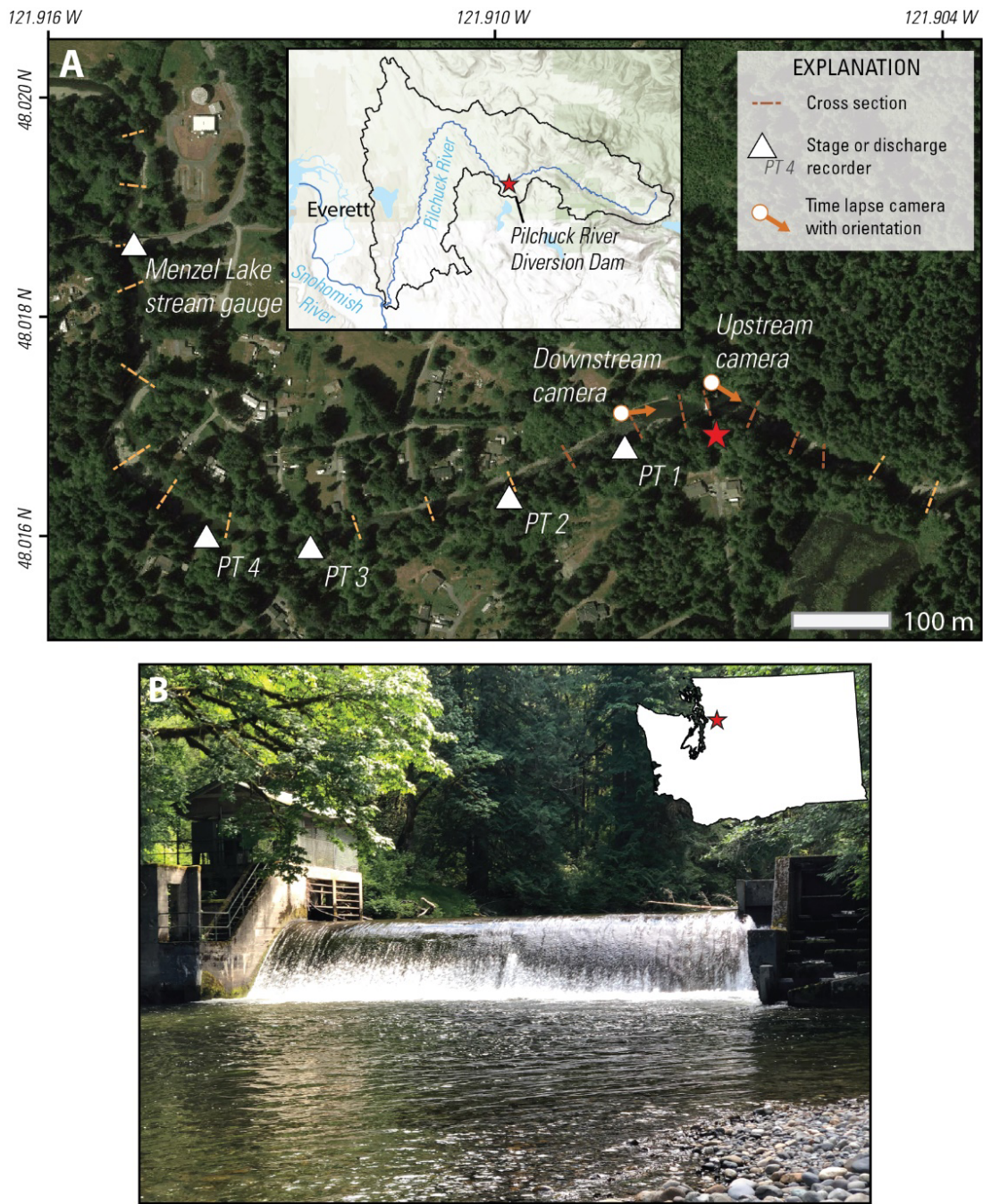
Figure 1. Site map of study area. A) Details of monitoring elements in reach near the Pilchuck Dam. Inset shows Pilchuck River watershed. Subset of cross sections resurveyed in September 2020 shown with darker coloring. Base map from Esri and its licensors, copyright
