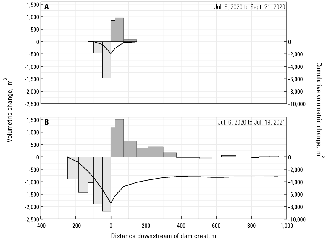
Figure 3. Volumetric channel change near the Pilchuck Dam site from A) July 6, 2020, to September 21, 2020, and B) July 6, 2020, to July 19, 2021. Volumes are based on repeat cross sections, using average end-area methods. Bars show volumetric change between sequential cross sections; black line shows longitudinal cumulative change starting from upstream-most cross section. All change in A was the result of manual grading during deconstruction.
