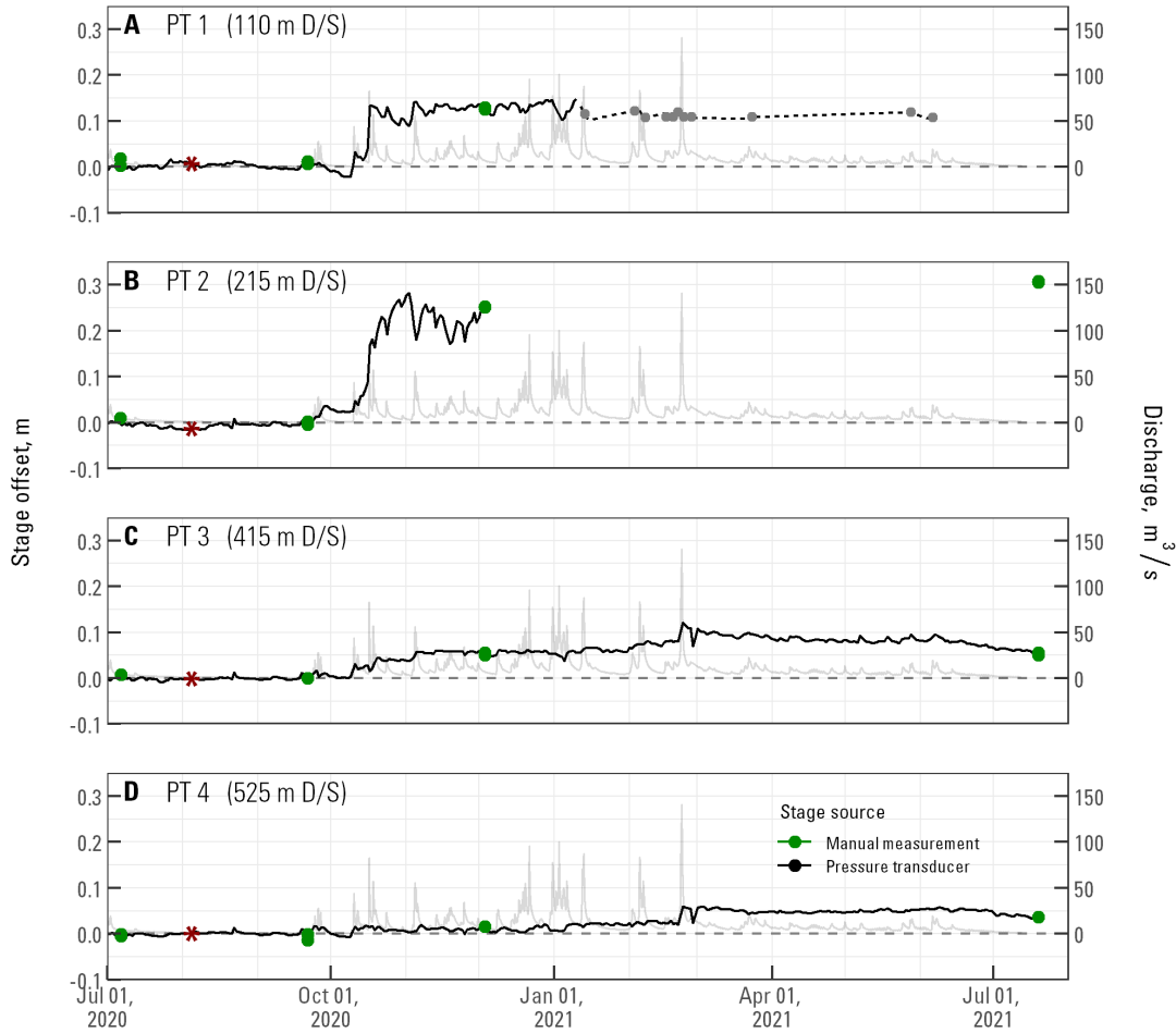
Figure 5. Stage offsets based on stage monitoring downstream of the Pilchuck Dam. Stage offsets provide an approximate measure of changes in mean channel bed elevation near the site of a given pressure transducer. Asterisks indicates timing of dam removal. Dashed line and points in A reflect analysis of PT 1 records after partial burial by sediment – see methods. Stage offsets based on manual stage measurements are shown (green points) to validate datum consistency at all sites and, for PT 2, to provide a point estimate of relative channel elevations at the end of the study.
