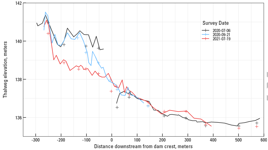
Figure 4. Approximate channel thalweg of the Pilchuck River before and after removal of the Pilchuck Dam. Lines represent total station longitudinal profile surveys; crosses are minimum elevations extracted from cross sections surveys.
